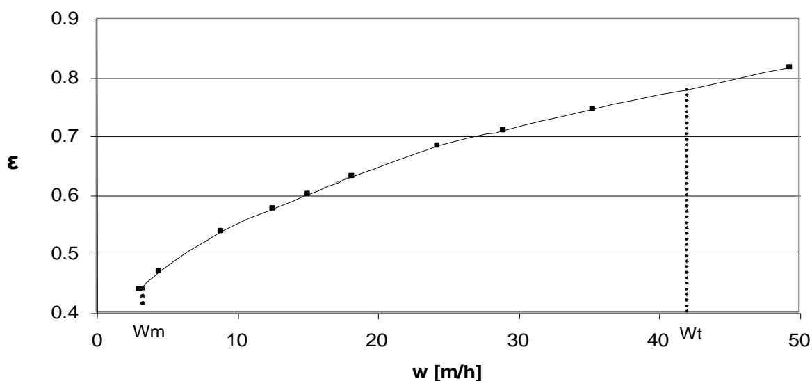
Fig. 3 Fluidized bed porosity
