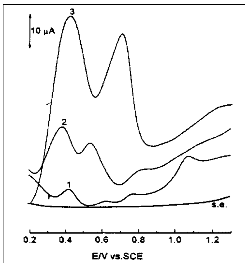
Figure 8. Square wave voltammogram of a DNA-biosensor in solution containing 4.5 \times 10^{-3} \text{ M} of MTX. Variation with time: (1) 0h; (2) 4h; (3) 96h. The electrode was kept in the solution between experiments. Supporting electrolyte (s.e.) 0.1 acetate buffer pH 4.5. Frequency 50 Hz.
