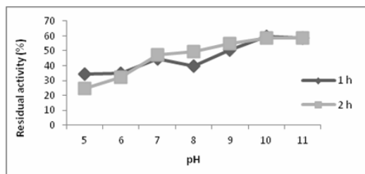
Figure 1. pH stability of LipS350-2.
