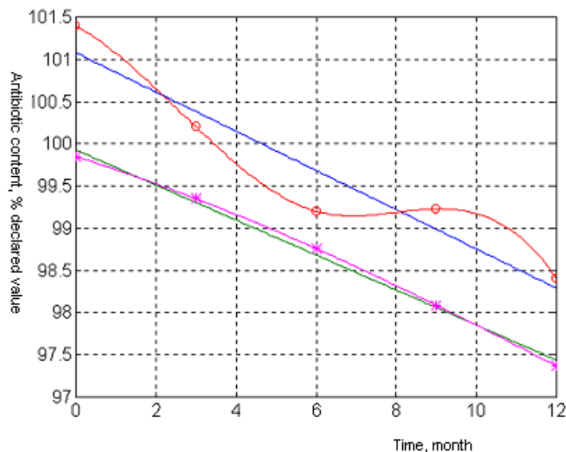
Figure 1. The degradation of active substances from powder under preservations conditions at 25°C for 12 months and the representation of regression equations.
